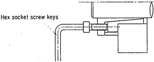
Fig. 4 Removal
