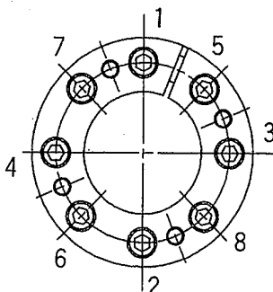
Fig. 3 Tightening sequence for bolts
