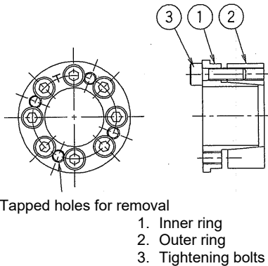
Fig. 1: Configuration
