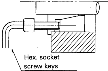
Fig. 4 Removal
