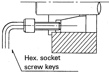
Fig. 4 Removal
