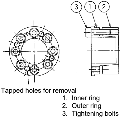
Fig. 1: Configuration
