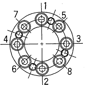
Fig. 3 Tightening sequence for bolts
