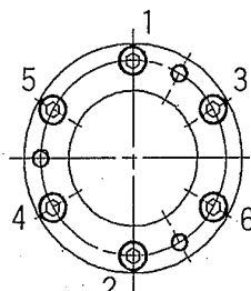
Fig. 3 Tightening sequence for bolts
