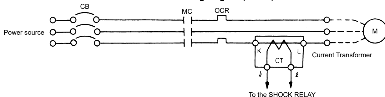
Standard Connecting Diagram (TSB50)
