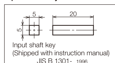
Input shaft key
