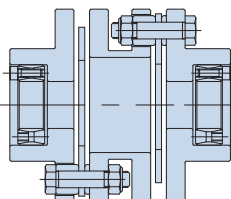
Example of coupling combined with AS Series POWER-LOCK
