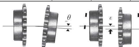
Angular misalignment
