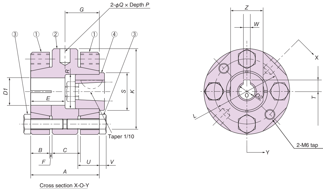
(1) Outer rings (2) Body (3) Pressure bolts (4) Adapter
