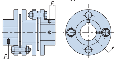
Standard hub/extended hub type
