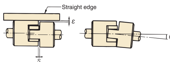
Figure 3. Centering
