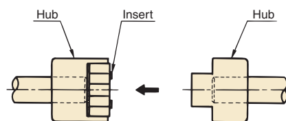
Figure 3. Centering
