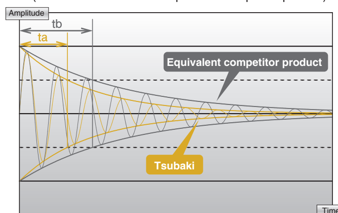
■ Example comparison of vibration damping characteristics (model LN28U98A1 and equivalent competitor product)
