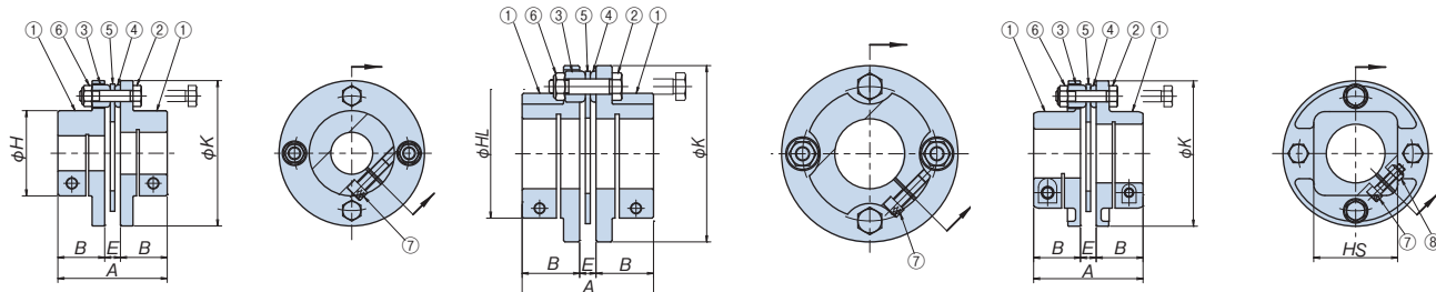
(1) Hubs (2) Reamer bolt (3) Washer (A) (4) Washer (B) (5) Disk (6) U-nut (7) Spacer
