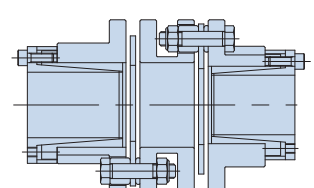
Example of coupling combined with TF Series POWER-LOCK
