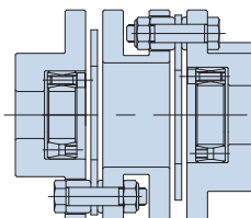
Example of coupling combined with TF Series POWER-LOCK
