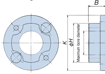
Enlarged hub
