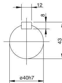
Detailed view of lateral/cross shaft ends
