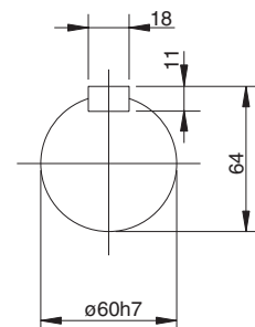
Detailed view of lateral/cross shaft ends
