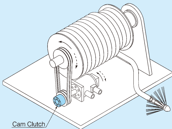
Application in pipe flusher
