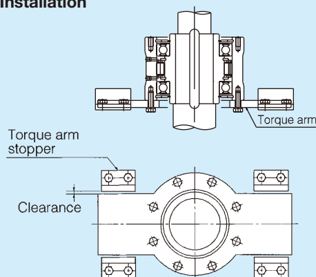
Installation example 2:
