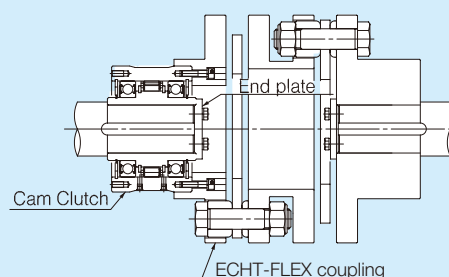
Installation example 3:
