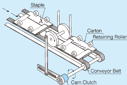
Automatic stapler example
