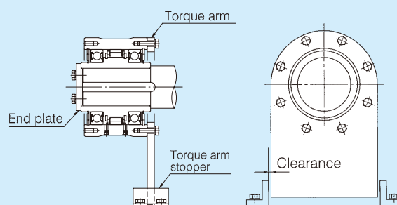
Installation example 1:
