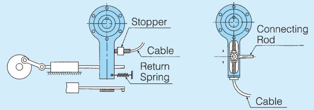
Structure of speed controlling section
