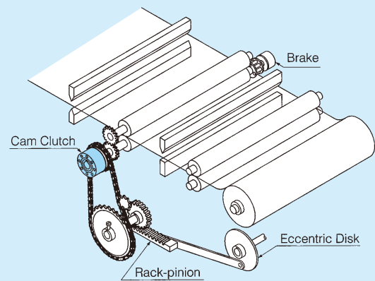
Feed roll example
