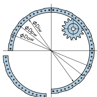
Inner drive pin wheel: NPF (4-segment model)
