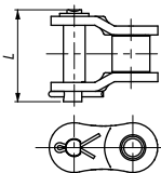
1-pitch offset link
