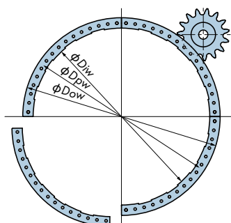
Outer drive pin wheel: GPF (4-segment model)
