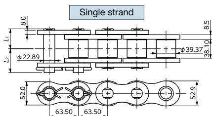
Connecting link
