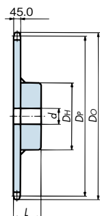
Welded construction 1B type
