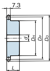
Hub without groove (13T and over)
